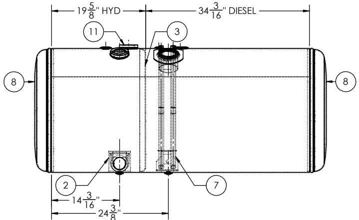
VIEWS FROM LEFT END OF TANK
