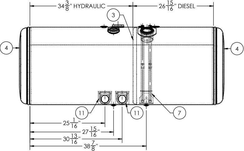
VIEWED FROM LEFT END OF TANK
