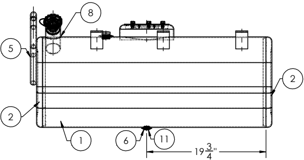
VIEW B-B SCALE 1 : 4 GASOLINE INTERNAL THREAD FILL NECK
