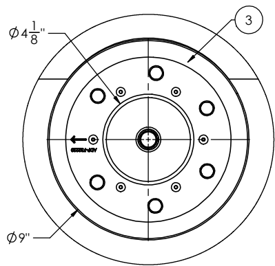
DETAIL A SCALE 1 : 3 GASKET REMOVED FOR CLARITY
