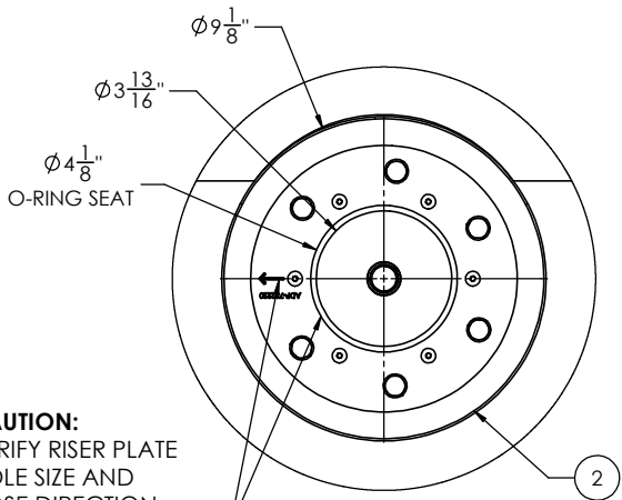
DETAIL A SCALE 1 : 3 GASKET REMOVED FOR CLARITY
