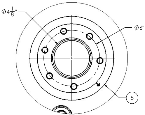
DETAIL A SCALE 1 : 3
